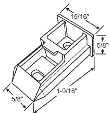
Part # Color 60-633 Natural 60-633B Black
