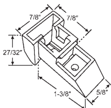
Part # Color 60-935 White 60-935B Black LAWSON
