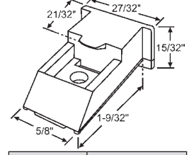
Part # Color 900-20576 White 900-20576B Black LAWSON
