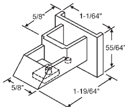
60-651A LH & RH Set SUGAR CREEK
