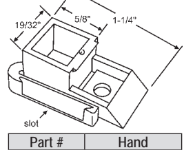
Part # Hand 60-605 Shown 60-606 Opposite Weatherstripping not included. IDA
