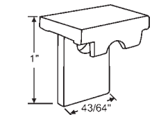
Part # Color 900-9500AW White 900-9500AB Bronze 900-9500AL Aluminum Aluminum SECURITY
