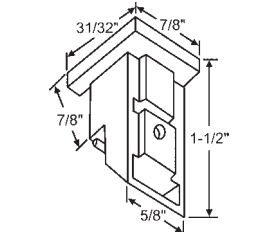
900-1852 3/16" dia. hole. Hole center up 17/32" from bottom.
