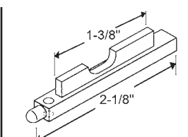
85-698 Bar Only. Die Cast BETTER-BILT
