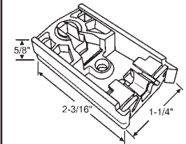
85-5016 POS Lock w/ Torque Plate
