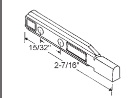
900-18821 RH (shown) and LH Set Die Cast
