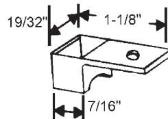
70-623 Nylon. Use with 72-500 Carrier and 72-603 Sash Clip
