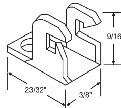
70-506 Metal Side Mount
