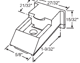
Part # Color 900-20576 White 900-20576B Black LAWSON
