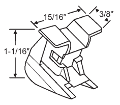
Suffix -12R 60-516 Bottom
