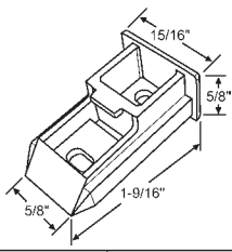
Part # Color 60-633 Natural 60-633B Black PGT 4000 SERIES
