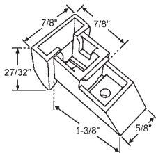
Part # Color 60-935 White 60-935B Black LAWSON
