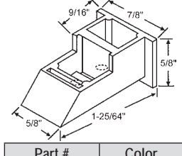
Part # Color 60-6004 White 60-6004BG Beige VBP / GENERAL ALUMINUM / BETTER BILT
