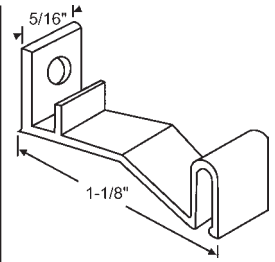
60-592 Metal Toggle. Used with 60-513B
